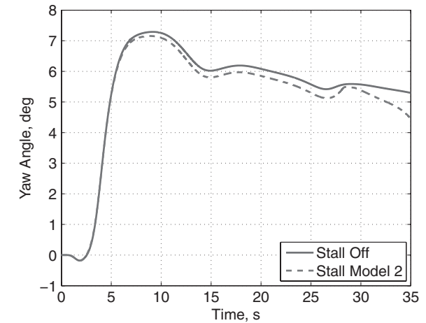
Fig. 37 Stall effects on B frame yaw angle (gust center amplitude: 10 m/s; duration: 4 s).
