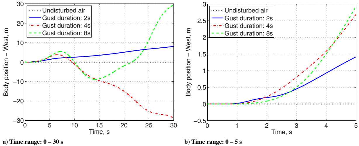
Fig. 22 Effects of gust duration on B frame lateral position.
