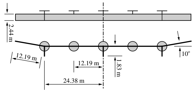
Fig. 11 Geometry of the flying wing model (after [4]).
