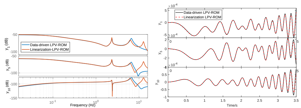
Figure 9. Comparison of frequency- and time-domain responses of data-driven ROMs and linearization-based ROMs at \alpha = 0^\circ .
