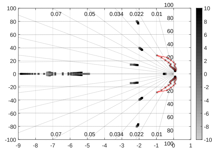
Figure 7. Root loci of ROMs of slender wing at grid points of the angle of attack.
