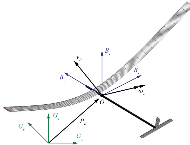
Figure 1. Flexible aircraft with large, nonlinear structural deformation.
