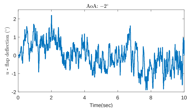
Figure 18. Control input to actively suppress the vibration.
