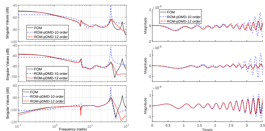
Figure 5. Frequency responses (left column) and time responses (right column) of u to y_1 (top), y_5 (middle), and y_{10} (bottom), with 10th- and 12th-order ROMs at the angle of attack \alpha = -10^\circ .
