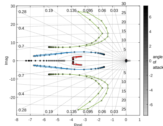
Figure 12. Root loci of ROMs of flexible aircraft at grid angles of attack.
