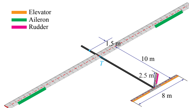
Figure 10. Platform of flexible vehicle.
