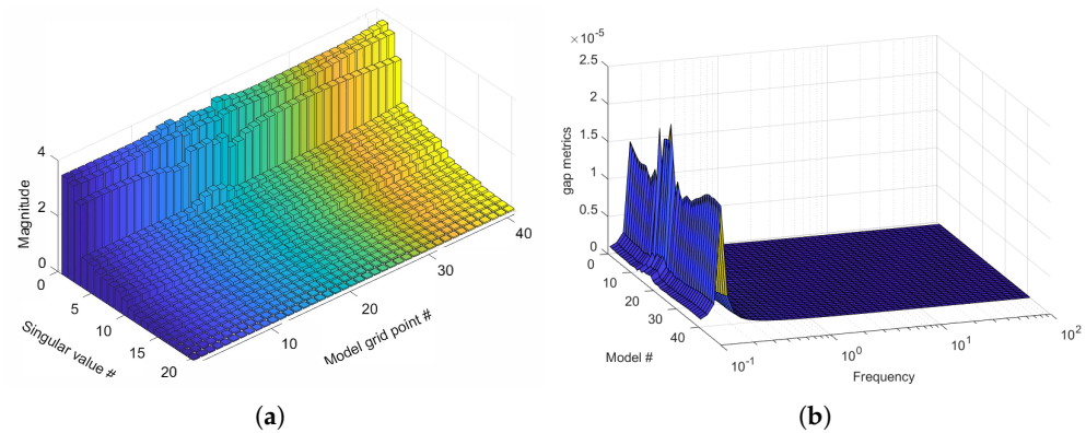
Figure 3. (a) Twenty largest singular values of grid models at fixed scheduling parameters; (b) v -gap metric surface of frequency responses at fixed models. A gap metric close to zero indicates that the two systems are dynamically similar. # indicates the index number.
