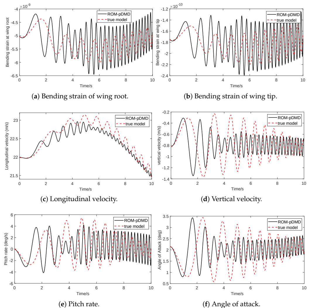
Figure 16. Time-domain responses of LPV-ROM and nonlinear FOM at non-equilibrium flight condition with sinusoidal input of 5 Hz.
