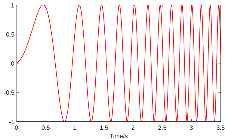
Figure 2. Excitation input (deflection angle in degree) of a chirp signal with sweep frequency from 0.1 to 10 Hz.
