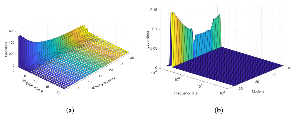
Figure 11. (a) Twenty largest singular values of flexible aircraft at fixed scheduling parameters. (b) v -gap metric surface of frequency responses of models at the grid angle of attack. Gap metric close to 0, meaning that two systems are similar.
