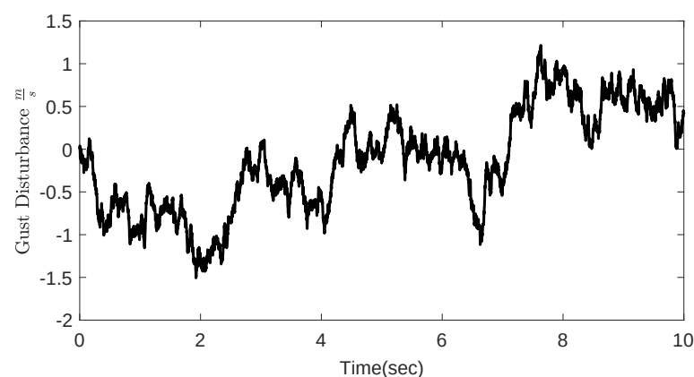
Figure 17. Profile of the Dryden gust disturbances to excite the flexible wing.
