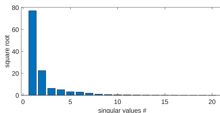
Figure 14. Square roots of 20 largest singular values of the parametric data-trace matrix. # indicates the index number.
