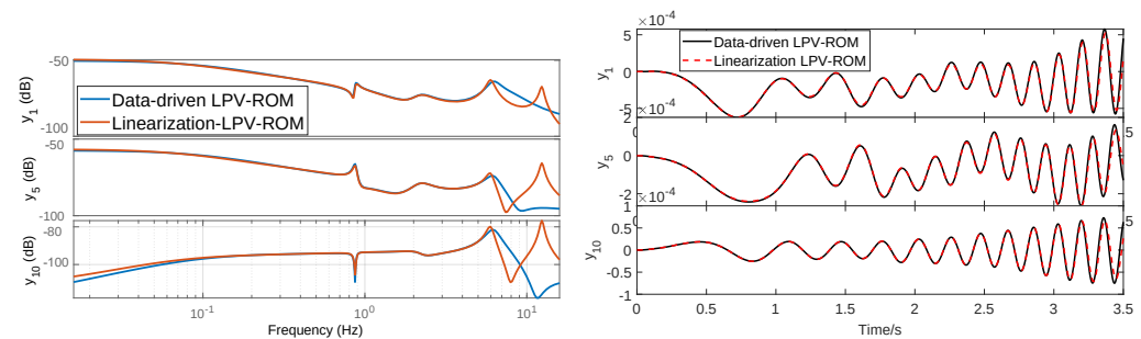
Figure 8. Comparison of frequency- and time-domain responses of data-driven ROMs and linearization-based ROMs at \alpha = -10^\circ .
