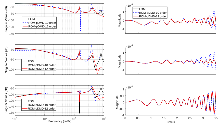
Figure 6. Frequency responses (left column) and time responses (right column) of u to y_1 (top), y_5 (middle), and y_{10} (bottom), with 10th- and 12th-order ROMs at the angle of attack \alpha = 0^\circ .
