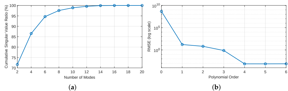
Figure 4. (a) Sensitivity study of cumulative singular value ratios with different model orders averaged across 41 grid models; (b) sensitivity study of polynomial order versus RMSE of strains on a logarithmic scale.
