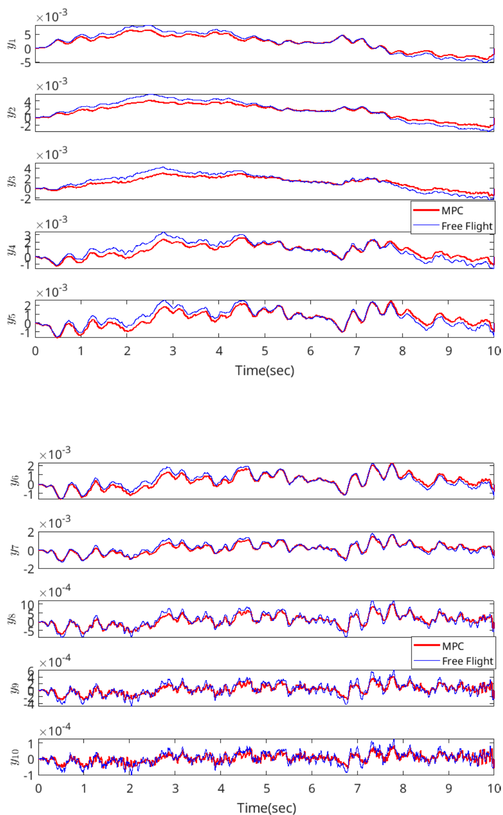
Figure 19. Comparison of time-domain bending strain responses for the MPC-controlled and uncontrolled systems.
