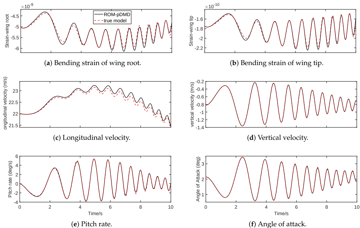
Figure 15. Time-domain responses of LPV-ROM and nonlinear FOM at non-equilibrium flight condition by chirp input of 0.1–2 Hz.
